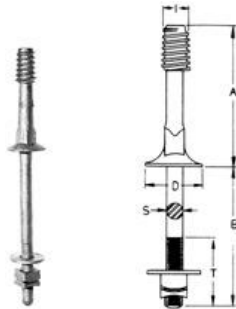
Long Shank Pins
